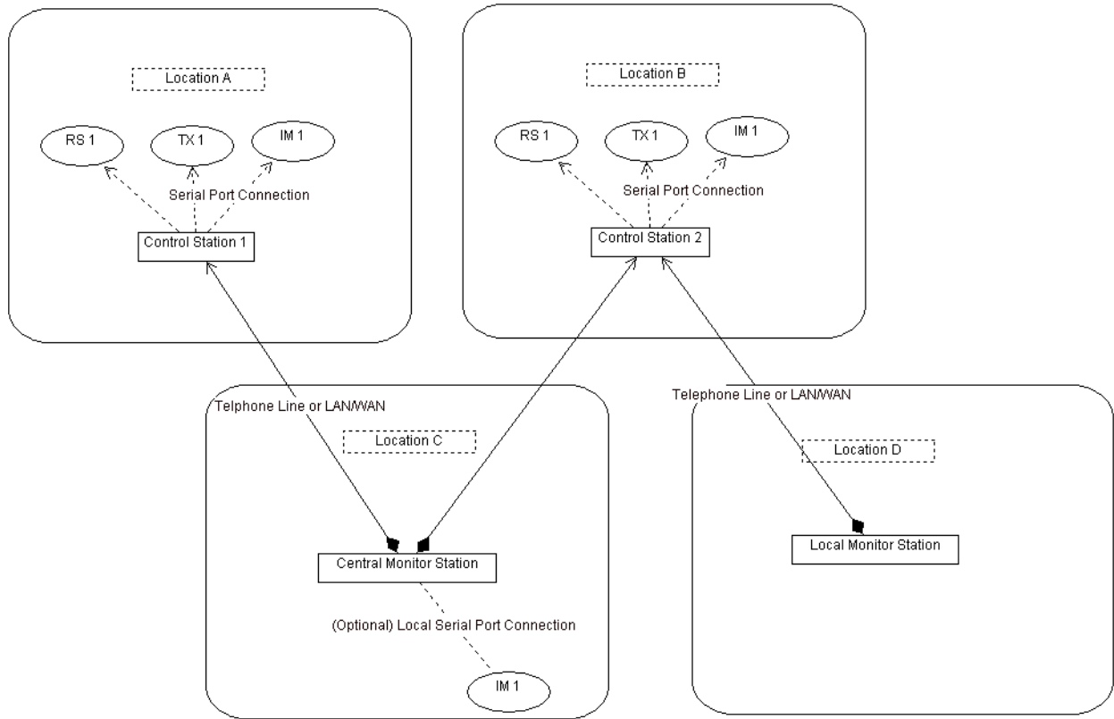
Central Monitor Station with 2 Control Stations and 1 Local Monitor
